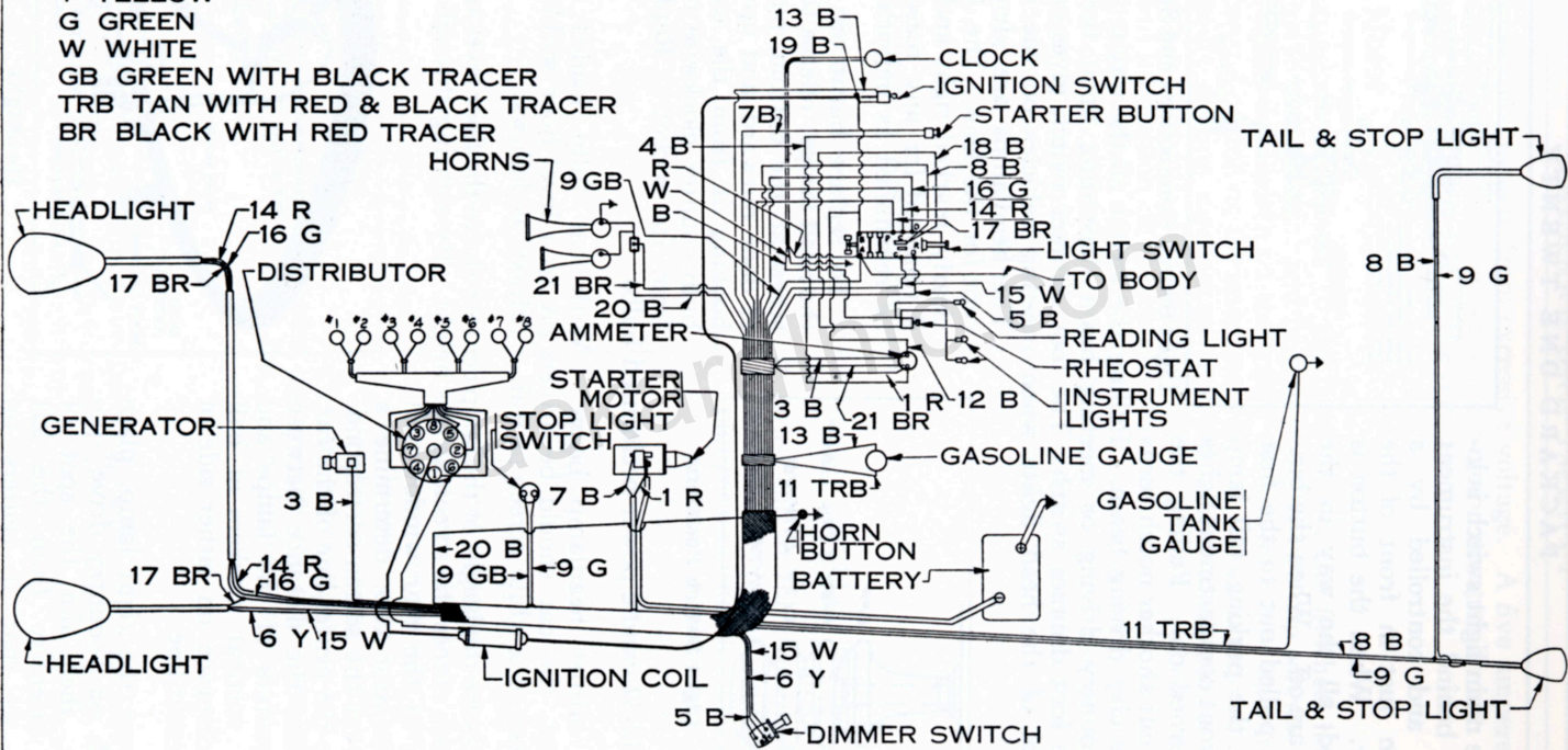
Wiring Diagram
